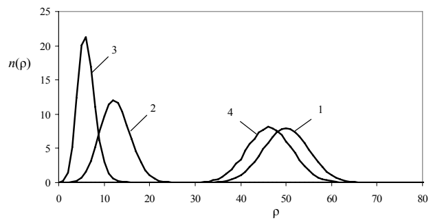
Fig. 2 – The distribution n(\rho) in the first generation of evolution: curve 1 is the distribution of \rho = \rho(S_{0k}, S_m) for the original genomes before learning, curve 2 is the distribution of \rho = \rho(S_{Fk}, S_m) for individuals after the learning, but before the selection, curve 3 is the distribution of \rho = \rho(S_{Fk}, S_m) for selected individuals, curve 4 is the distribution of \rho = \rho(S_{0k}, S_m) for the genomes of selected individuals at the end of the generation (results are averaged on 10,000 calculations)
