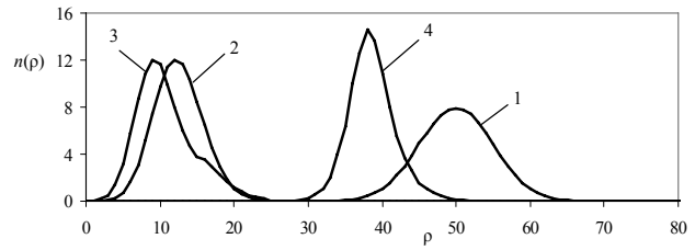
Fig. 4 – The distribution n(\rho) in the first generation of evolution, the fitness of individuals is determined by the expression (2): curve 1 is the distribution of \rho = \rho(\mathbf{S}_{0k}, \mathbf{S}_m) for the original genomes before learning, curve 2 is the distribution of \rho = \rho(\mathbf{S}_{Fk}, \mathbf{S}_m) for individuals after the learning, but before the selection, curve 3 is the distribution of \rho = \rho(\mathbf{S}_{Fk}, \mathbf{S}_m) for selected individuals, curve 4 is the distribution of \rho = \rho(\mathbf{S}_{0k}, \mathbf{S}_m) for the genomes of selected individuals at the end of the generation; the displacement of the distributions to smaller values \rho is significantly faster than in Fig. 2 (results are averaged on 10,000 calculations)
